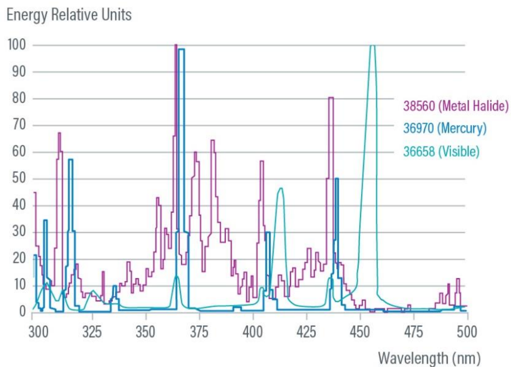
Figure 36. ECE Flood Lamp Spectral Output
