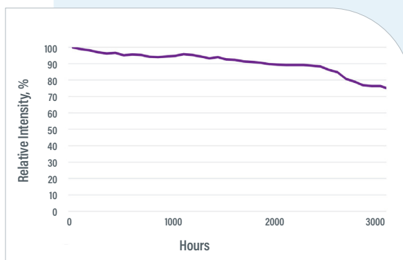
Figure 6. LED Degradation Testing - RediCure®
