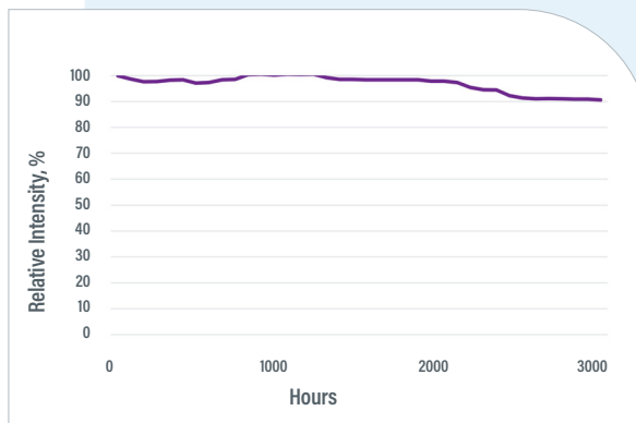
Figure 8. LED Degradation Testing - VisiCure®
