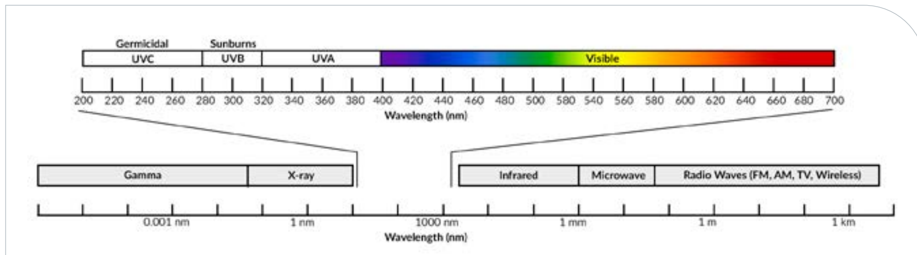
Electromagnetic Spectrum
