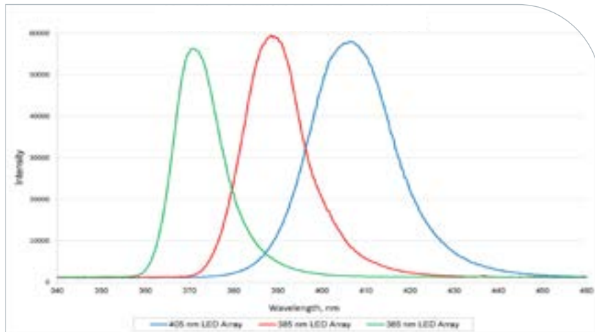
Example of a Light-Curing System Spectral Output Chart
