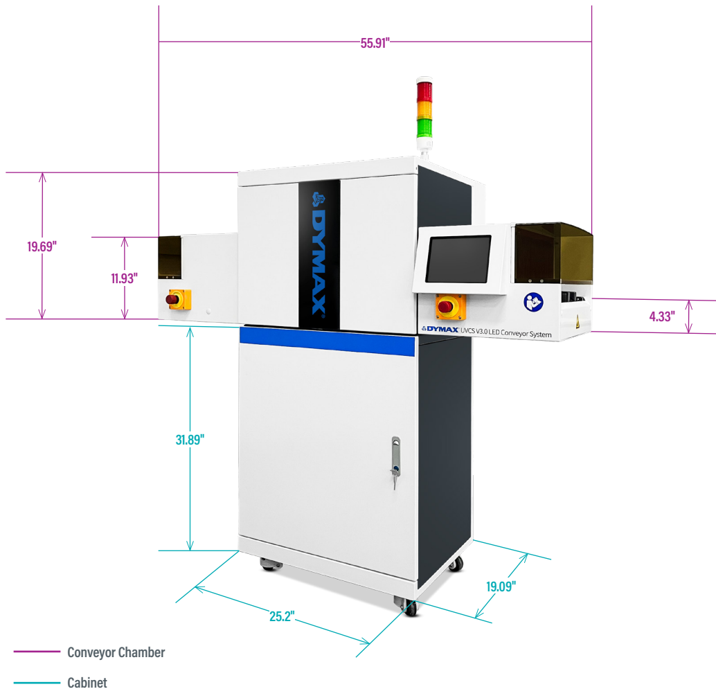
Figure 3. UVCS V3.0 LED Dimensions
