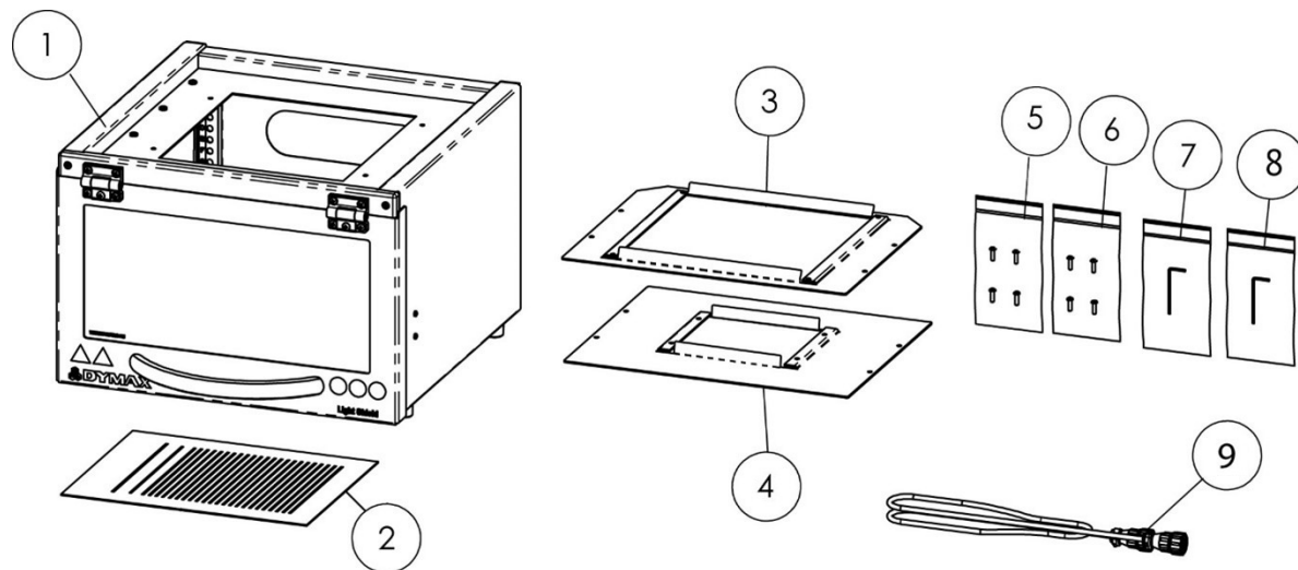
Figure 2. Light Shield (PN 41175) Components
