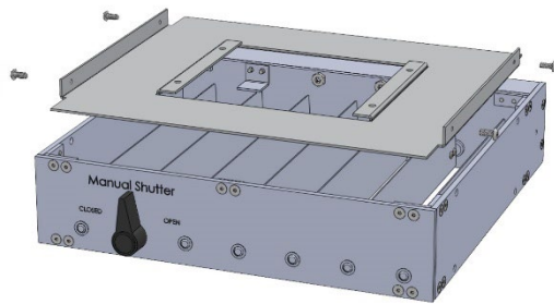
Manual Shutter
