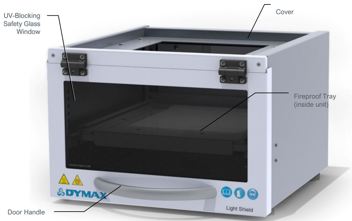
Figure 1. Main Components of the EC Light Shield
