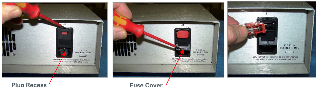
Figure 16. Replacing Fuses in the Power Supply
