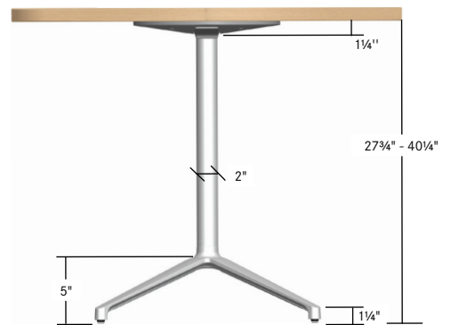
Elevation View of Story Base
