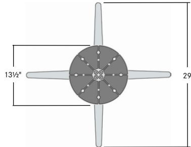
Plan View of Story Base
