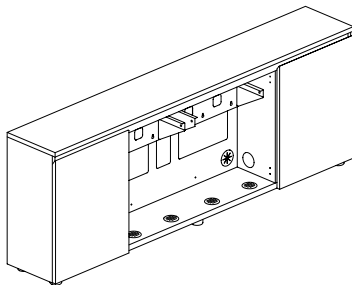
Front View (Shown without doors)
