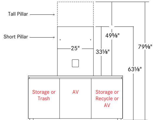
Three Door Credenza
