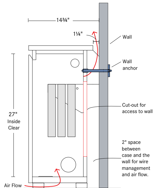
Section view showing relationship of credenza to wall.
