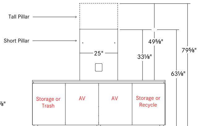
Four Door Credenza
