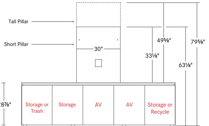
Five Door Credenza
