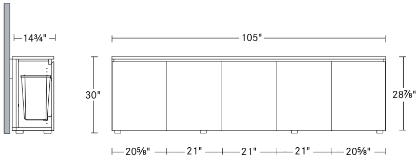
End View
