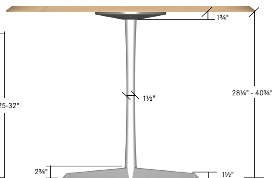
Elevation View of Vue Base
