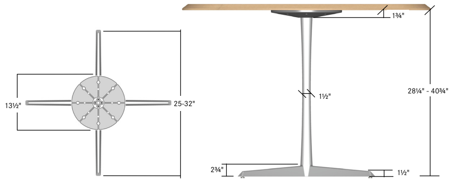
Plan View of Vue Base
