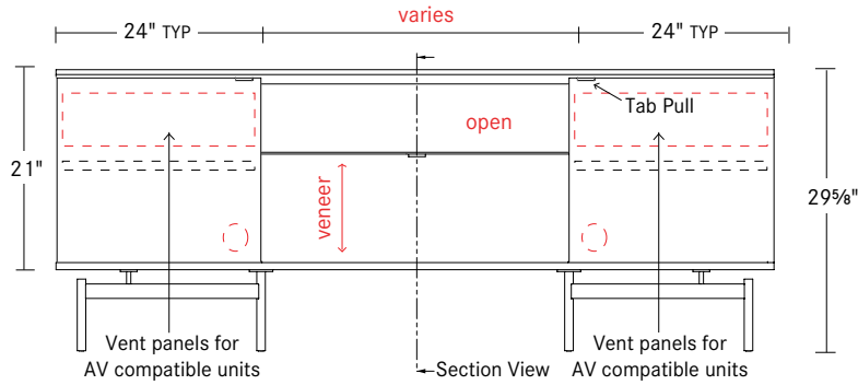
Front View
