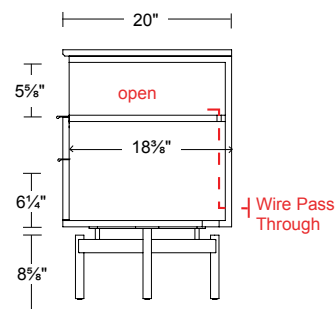
Section View
