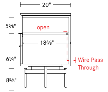
Section View
