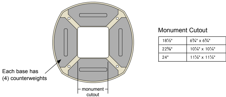
Top view showing monument cutout and counter weight details
