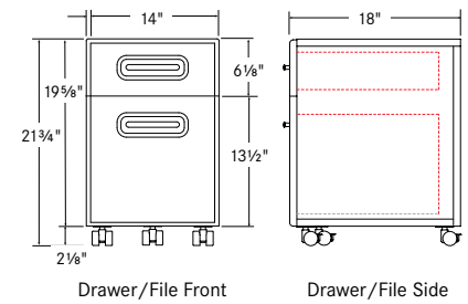
Drawer/File Front
