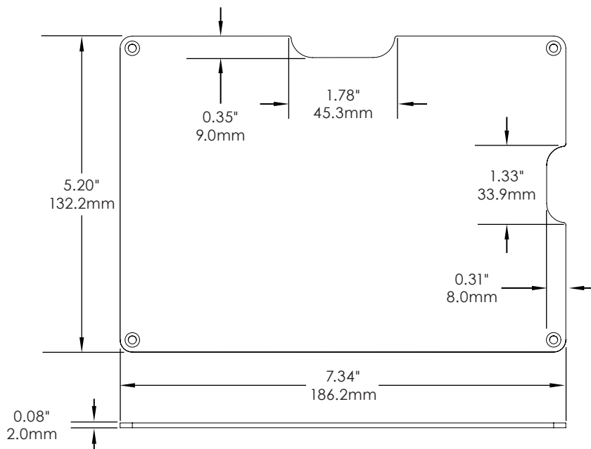
Honeywell EDA10 Rear Cover (CT1514):
