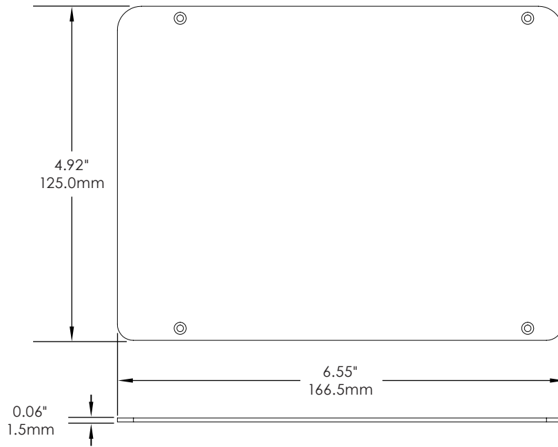
Zebra ET40/45 Battery Cover (CT1512):
