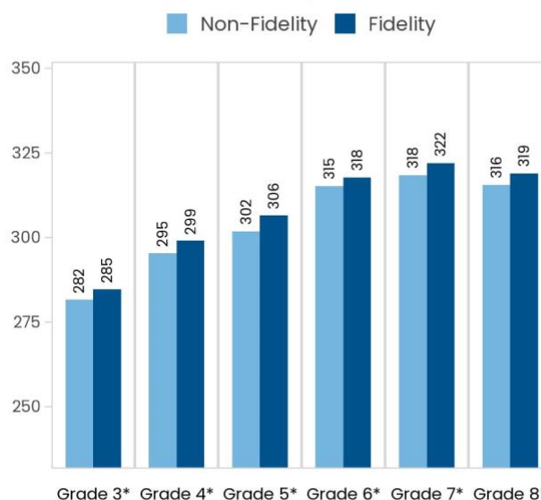
FAST Mathematics Scores by Fidelity Use
