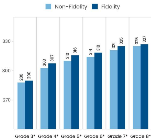
FAST Reading Scores by Fidelity Use
