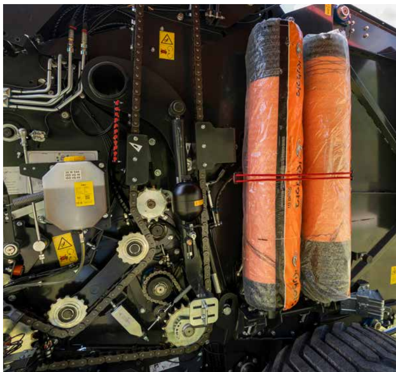
The vertical net roll storage gives an easy access to the transmission of the baler.
