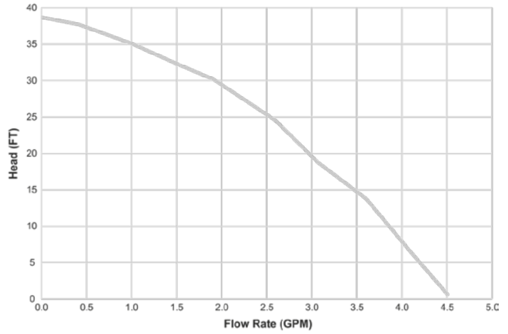
PUMP PERFORMANCE
