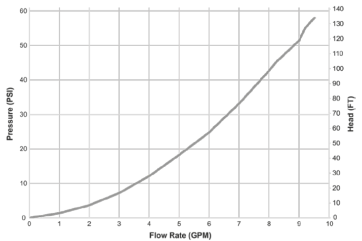
PRESSURE LOSS
