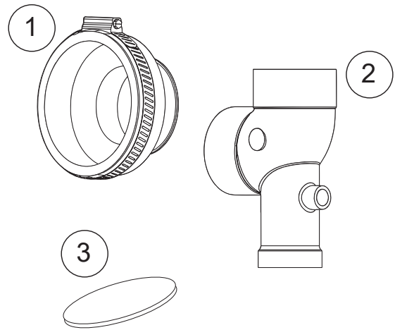
Figure 9. 4" Exhaust Elbow Fittings
