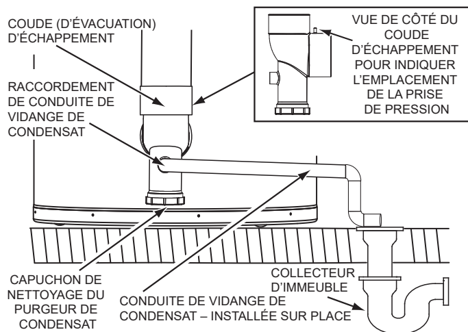
Figure 15. Coude d'évacuation/condensat
