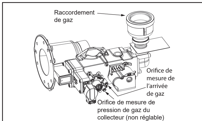
Figure 76. 119 gallons - Vanne de gaz
