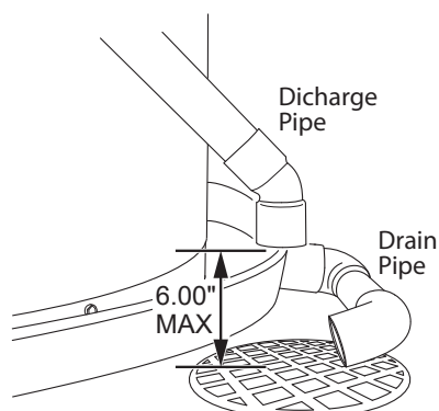
Figure 14 - The end of the T&P Relief Valve discharge pipe must stop no more than six inches above a floor drain or terminate outside the building.
