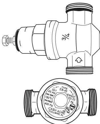
Figure 16 - A Pressure Reducing Valve is required if your home's water pressure is above 80 psi.
