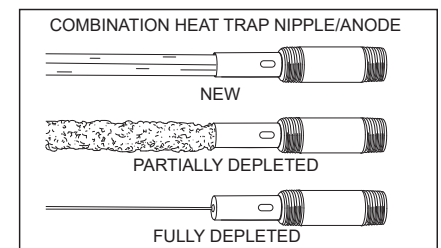
Figure 29 - Combination heat trap nipple/anode rods from new (top) to partially depleted (middle) to fully depleted (bottom).
