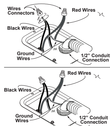
Figure 20 - Connecting the electrical wires.
