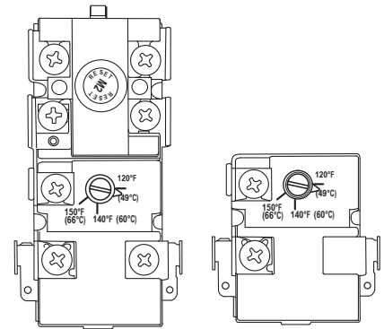
Figure 37 - Upper and Lower Thermostats
