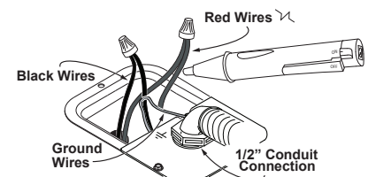
Figure 34 - Non-Contact Circuit Tester
