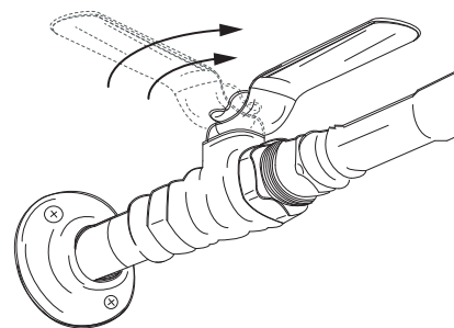
Figure 18 - Fully open the cold water supply valve.
