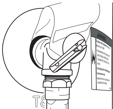
Figure 13 - The T&P Relief Valve discharge pipe must be installed properly and piped to an adequate drain.
