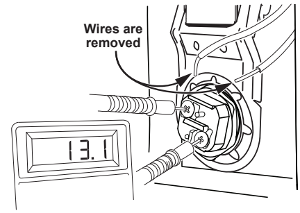
Figure 23 - Use a multimeter to check the resistance of the upper heating element.
