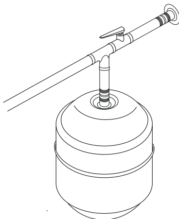
Figure 17 - The Thermal Expansion Tank should be pressurized with air, to match the home's incoming water pressure.
