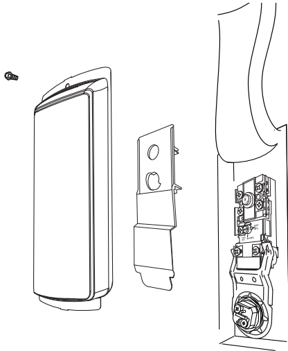
Figure 35 - Access Panel
