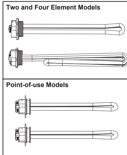
Figure 31 - Heating Element (with gasket)
