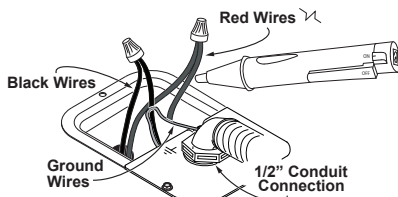
Figure 30 - Non-Contact Circuit Tester
