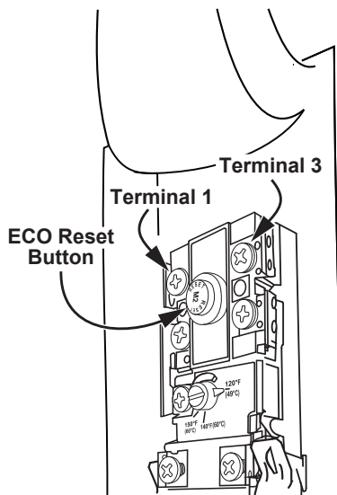
Figure 24 - Energy Cut Off (ECO) button
