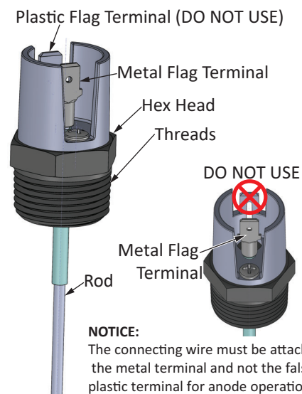
Figure 8: Top of new anode
