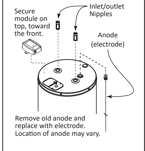
Figure 5: Top view of electric water heater.
