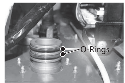
Figure 80 - Gas inlet connector O-rings
