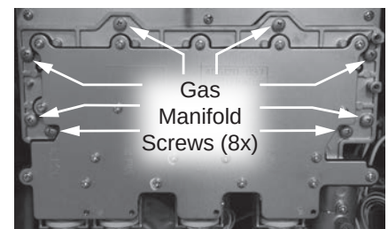
Figure 159 - Removing gas manifold from old primary heat exchanger
