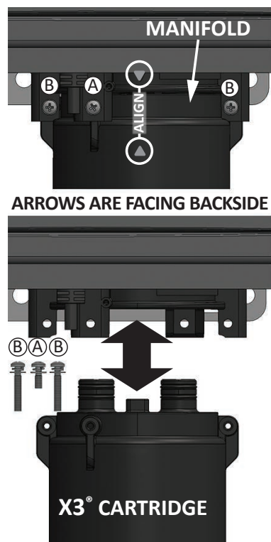
Figure 8 - X3® Cartridge
