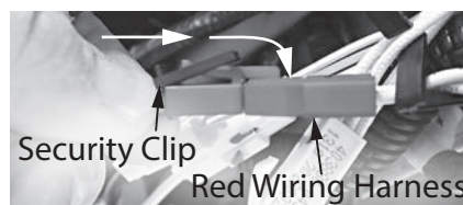
Figure 200 - Reconnecting the wiring harness
