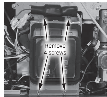
Figure 121 - Removing UIM and bracket screws
