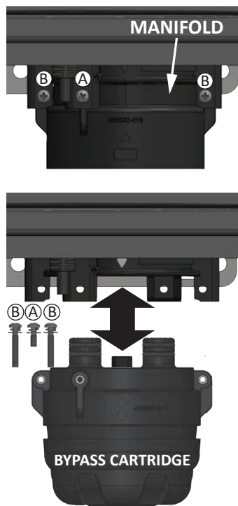
Figure 9 - Bypass Cartridge
