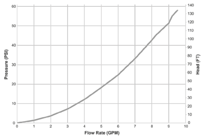
PRESSURE LOSS
