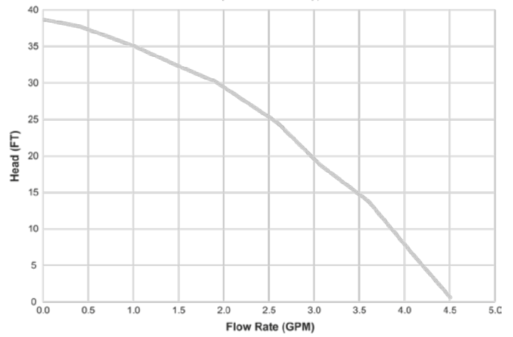
PUMP PERFORMANCE
