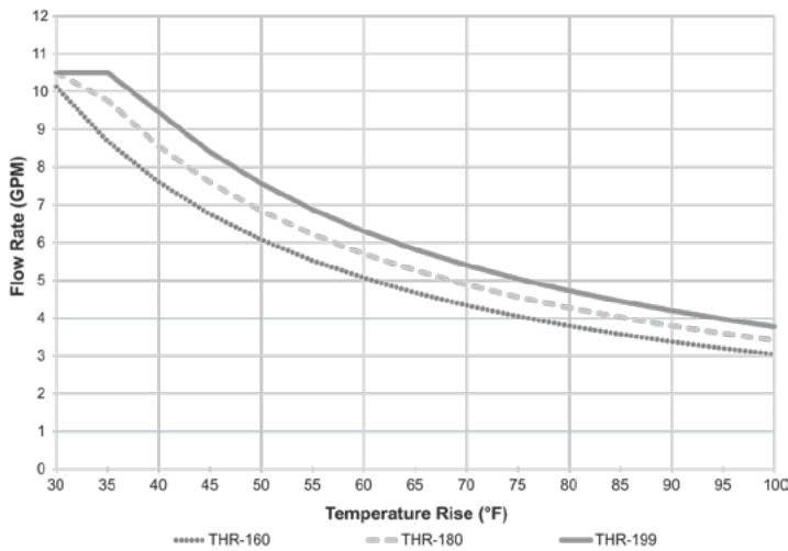
FLOW RATE
