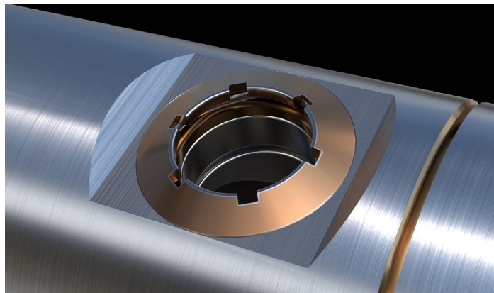
eRED® valve flow port
