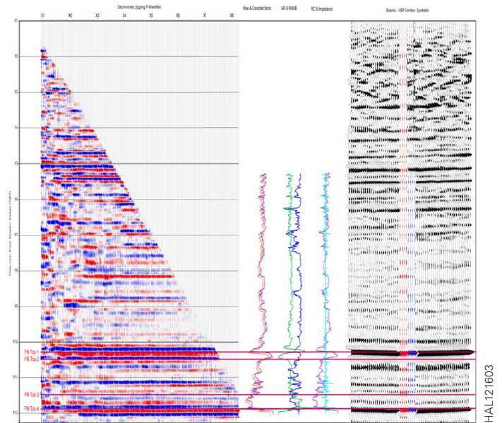
Zero-Offset VSP Imaging
