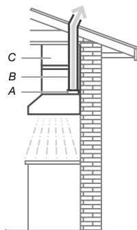
Descarga Vertical
