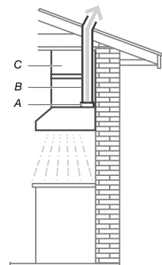
Vertical Discharge
