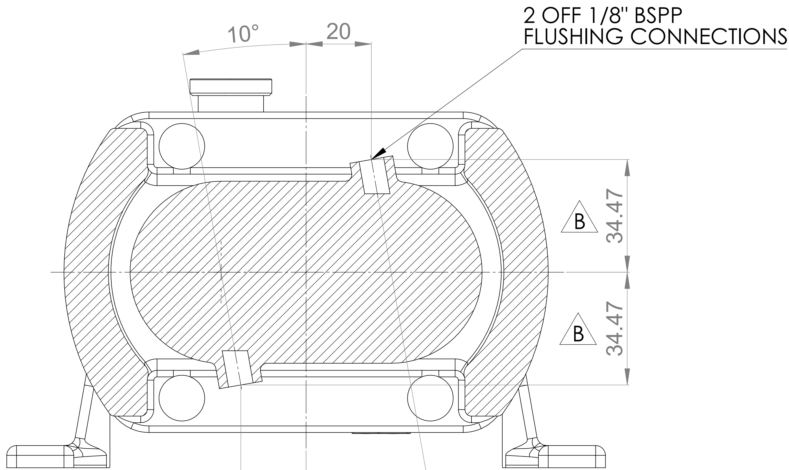
SECTION B-B
