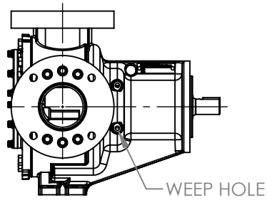
VIEW B-B SCALE 1 : 10
