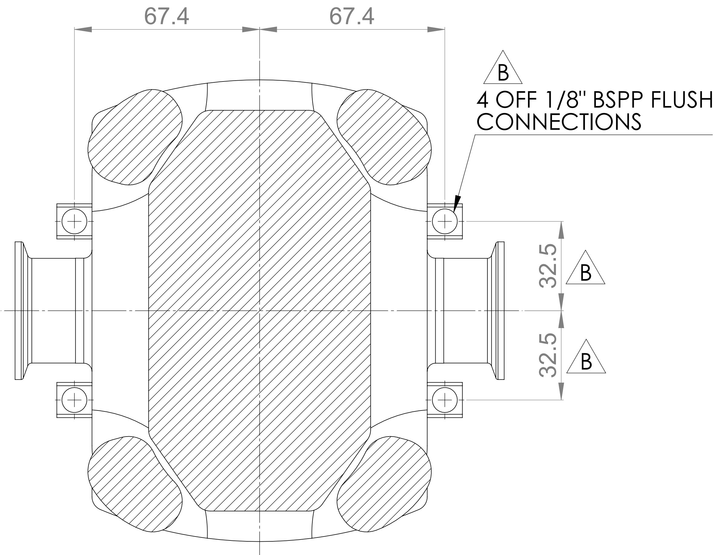
SECTION B-B
