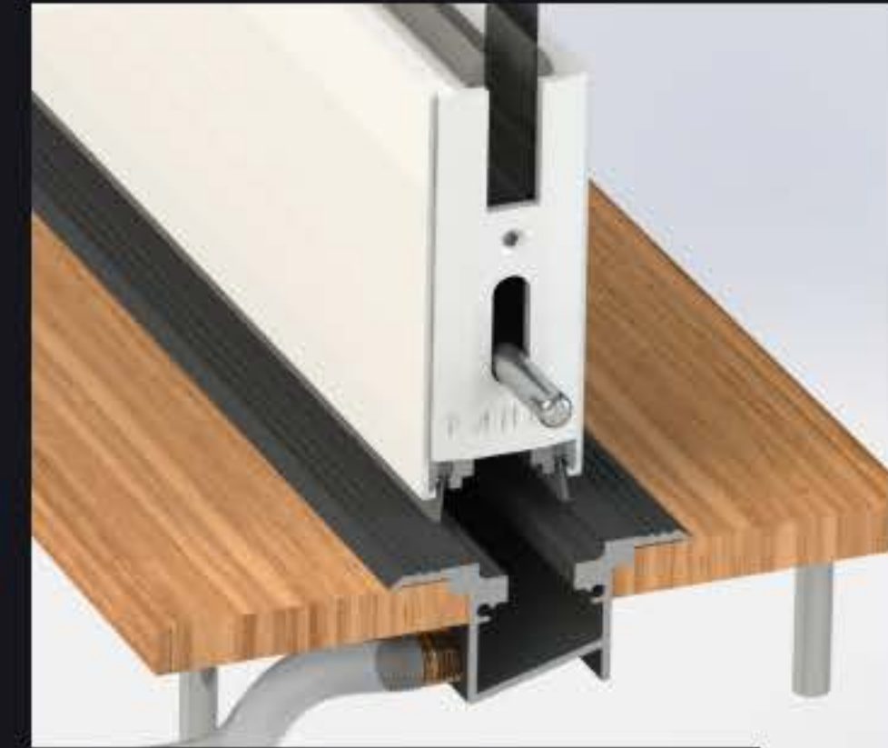
1 1/2" Recessed Drainage Track
