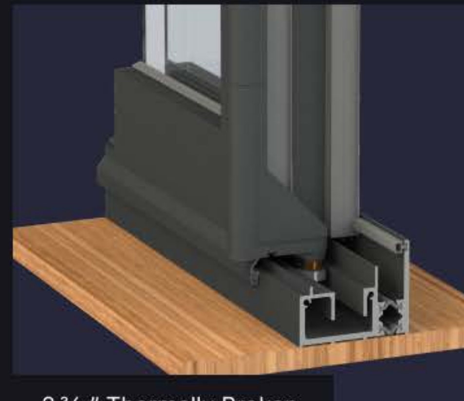
2 3/16" Thermally Broken Standard Surface Track
