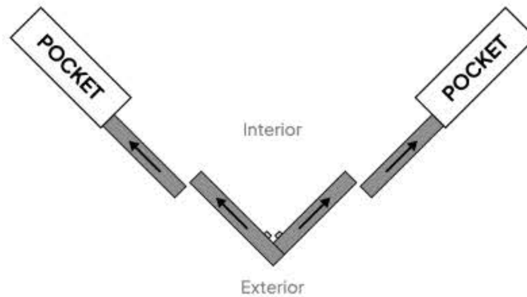
Zero-Post Corner
