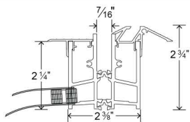
1 3/16" Recessed Track Bottom Running (FTS.77 and FUTS.77 only. Thermally Broken)
