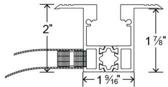
7/16" Recessed Track Bottom Running (FTS.77 and FUTS.77 only)
