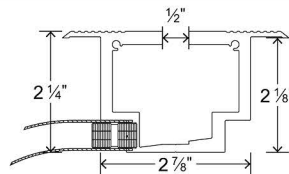
3/4" Recessed Track
