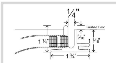
5/8" Surface Track Exclusive to SS.90 systems
