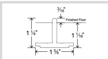
5/8" Surface Track with Sill Pan SIS.81 and STS.83 only. Optional ramps available
