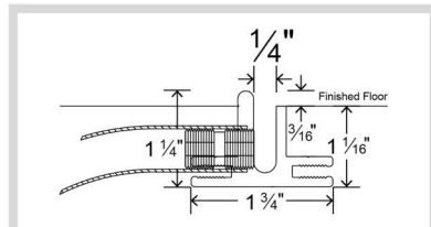
9/16" Surface Track Exclusive to SS.90 systems
