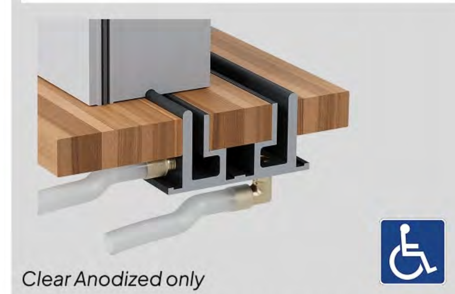
2 1/2" ADA Recessed Drainage Track (with Retention Track)
