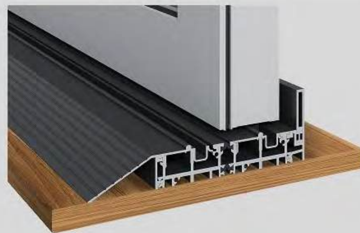
1 1/8" Surface Drainage Track Exclusive to NOVA.LS systems
