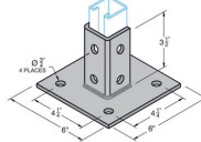
Post Base
