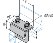
Beam Clamp
