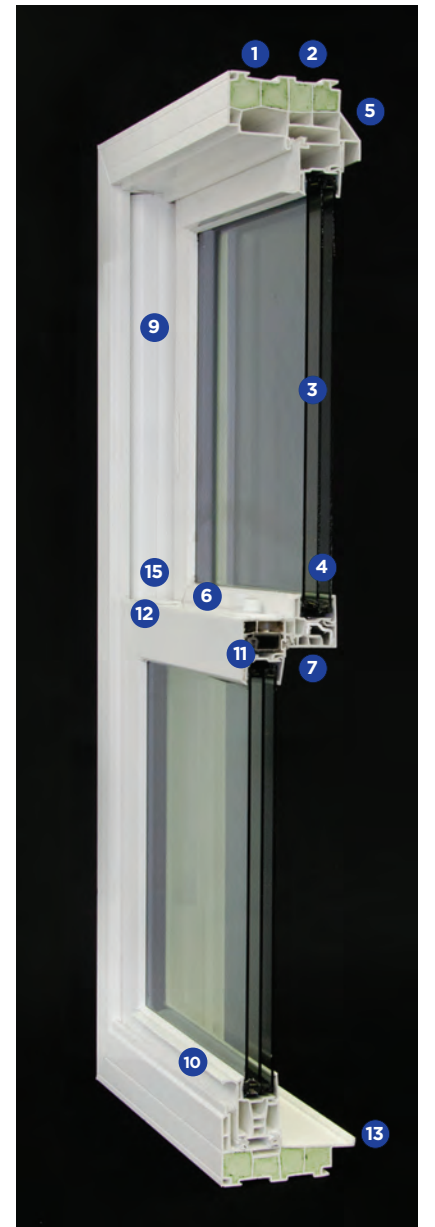
Triple-pane glass and a foam-enhanced mainframe results in superior thermal performance.
