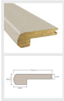
Stair Nose
