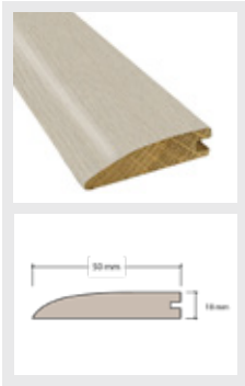
Reducer
