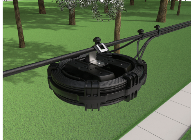
Back-to-Back Stacking of SLACKLOOP Drop Cable Storage (Aerial Applications ONLY)
