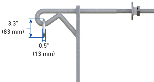
7/8" Shield Wire Bracket with 1/2" Chain Link
