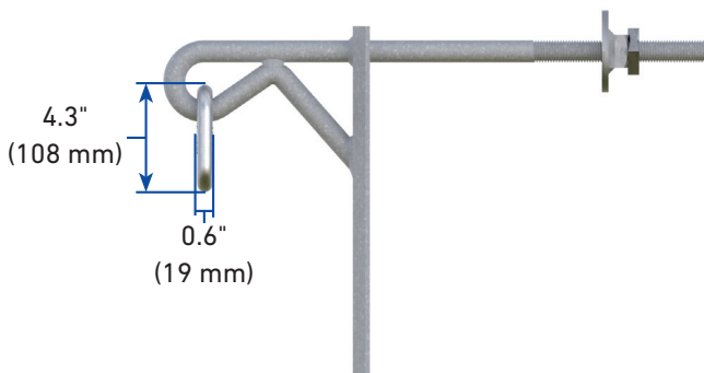
7/8" Shield Wire Bracket with 5/8" Chain Link
