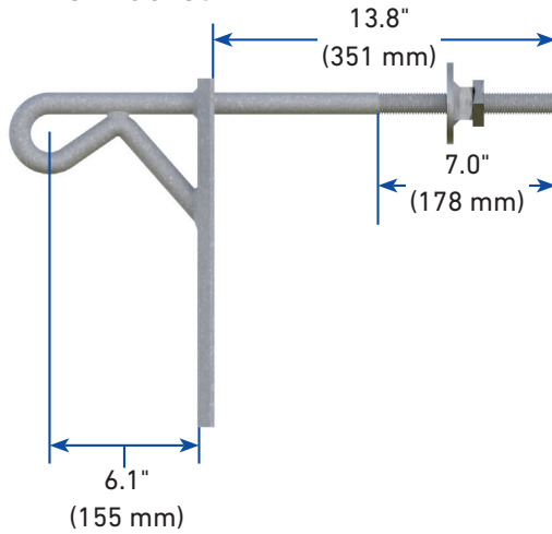
7/8" Shield Wire Bracket with 1/2" Chain Link
