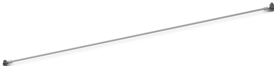
5 ft (1.5 m) Long 95mm 2 (19W) Aluminum Ground Wire Assembly (Catalog Number: 710011205)
