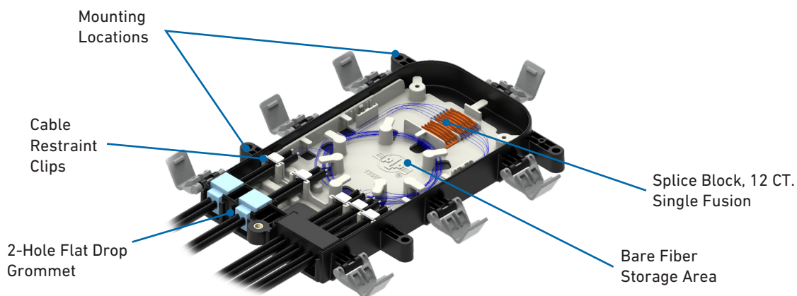
Drop Organizer STP-L Contact PLP for more information
