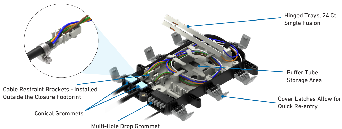
Universal Organizer STP-L
