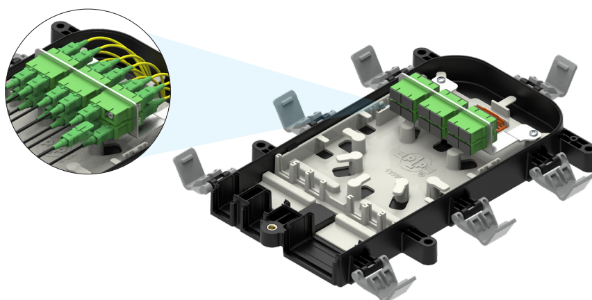
STP-L3 with Standard Bulkhead and Adapters Contact PLP for more information
