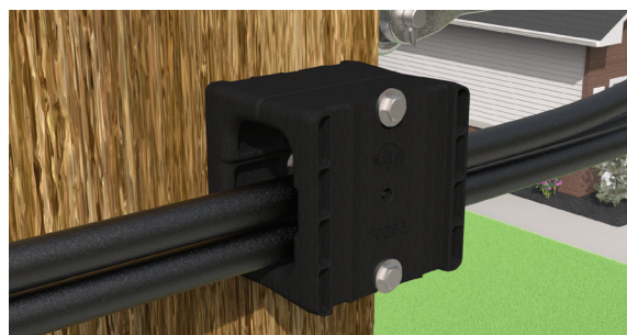
Uni-Group Cable Guide Installed on Wood Pole
