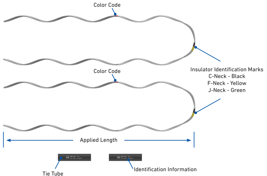
Double Side Tie Assembly
