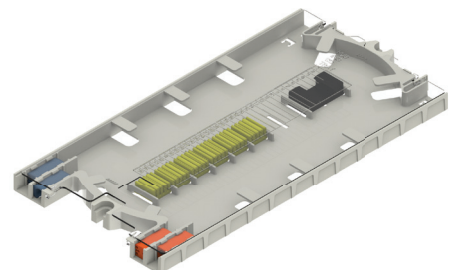
COYOTE LITE-GRIP Long Deep Profile Splice Tray Kit for Single Fusion Splices & 1x32 Pre-Connectorized Splitters (48 Splice CT.)
