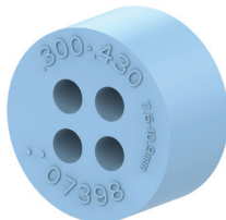
For Cable Diameters 0.30" – 0.43" (7.6 – 10.9 mm) Catalog Number: 8003664
