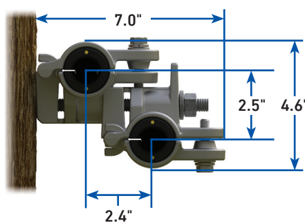
Stacked FAS
