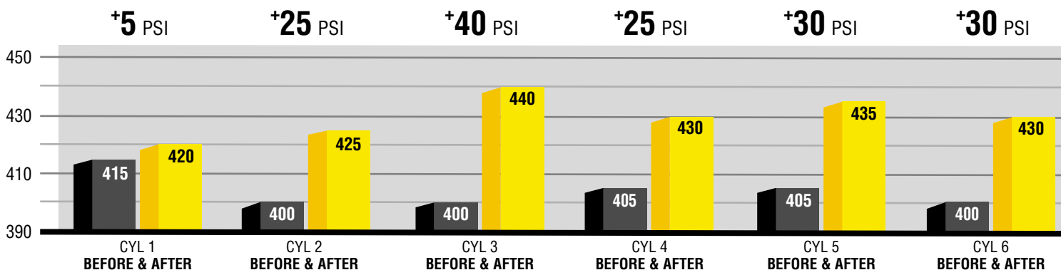
COMPRESSION RESULTS: Compression was restored across all cylinders after the BG service was performed.
