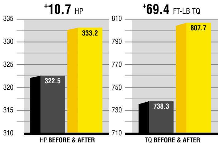
DYNO RESULTS: HORSEPOWER & TORQUE
