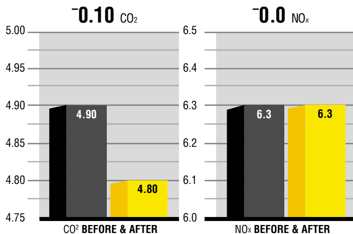
TAILPIPE EMISSIONS RESULTS: CO 2 & NO x
