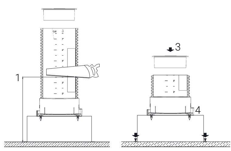
Optional Steps for Trimming Device Height
