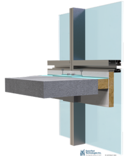
Zero Spandrel/All Vision Glass
