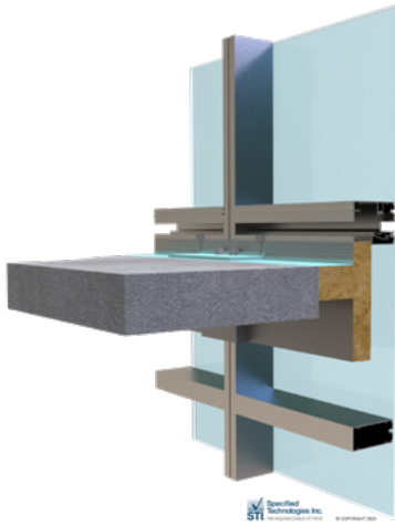
Valance Spandrel Panel
