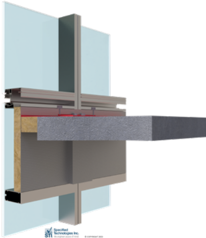
Insulated Spandrel Panel
