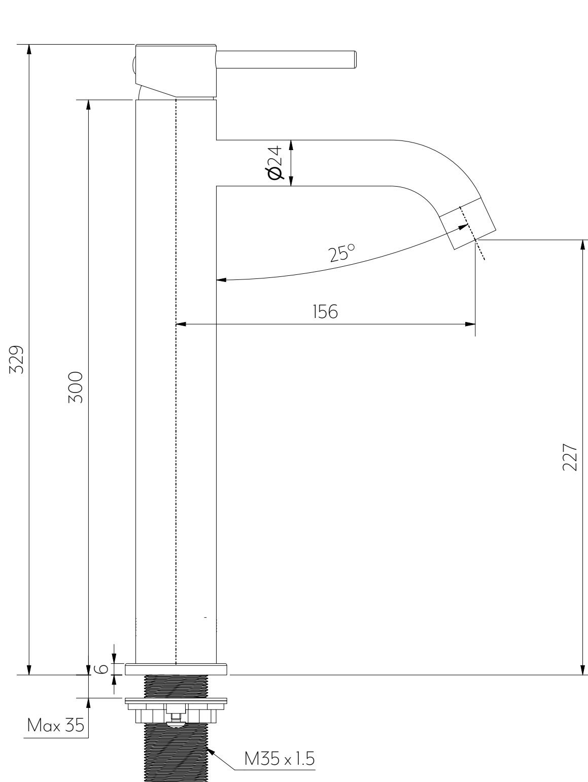
Side View
