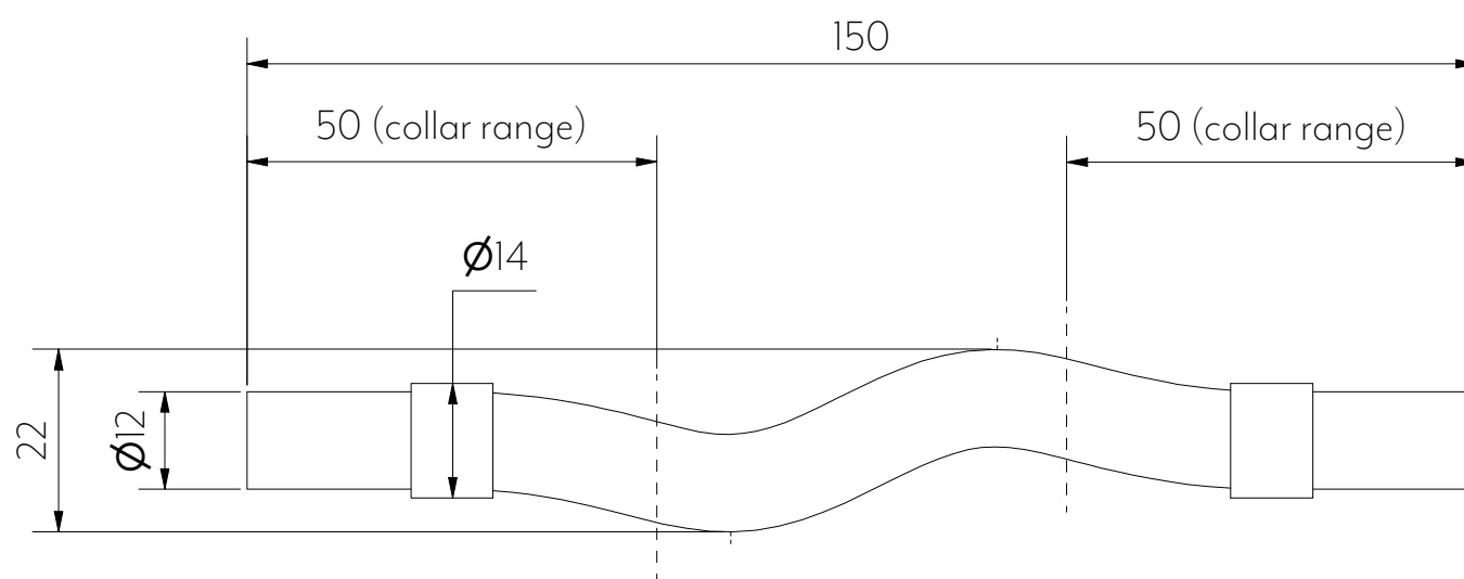
Front View
