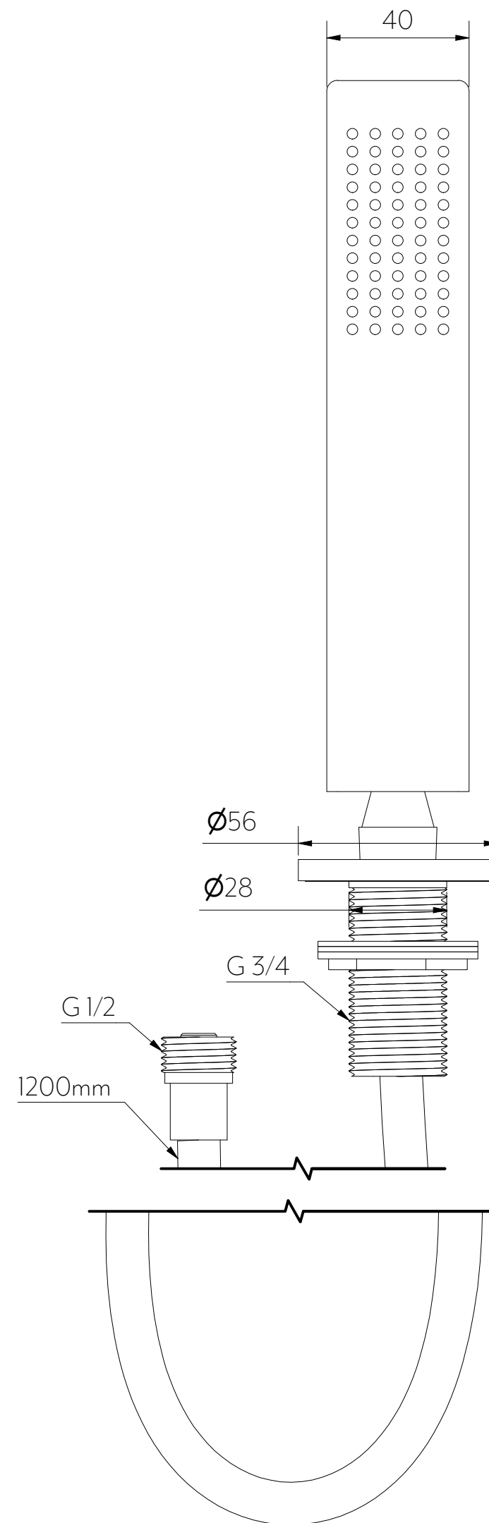
Front View
