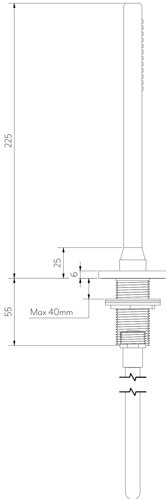
Side View
